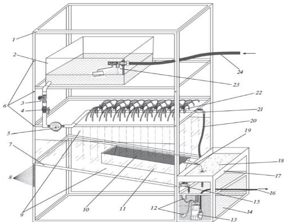
Figure 1: Sprinkler installation diagram
