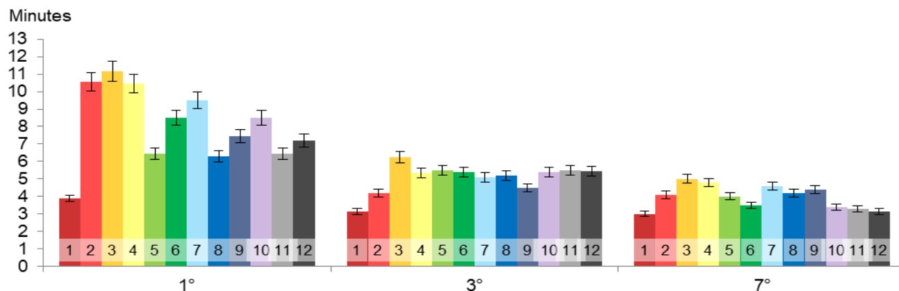
Figure 2: Time of appearance of surface runoff depending on angle of inclination and doses of FG and TL
