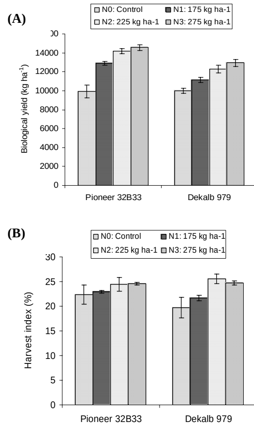
Figure 3(A, B). Interactive effect of maize hybrids and different nitrogen levels on biological yield (A) and harvest index (B) of maize hybrids under saline conditions \pm SE
